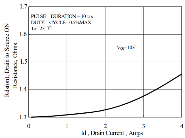
Fig 2 Drain Current
